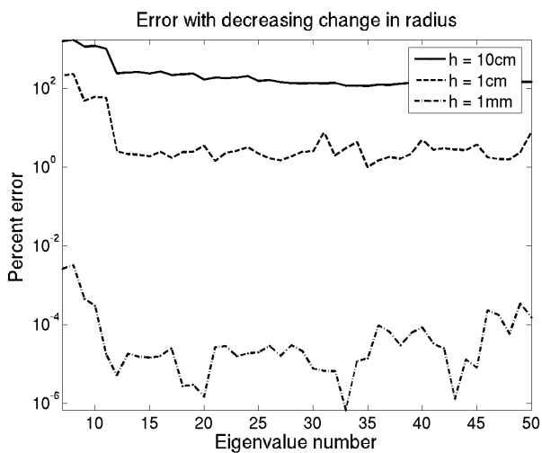
Figure 15: Error for different size h . 8 planes of symmetry.
