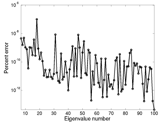
Figure 6: Error for h = 10\text{cm} . Larger subspaces.
