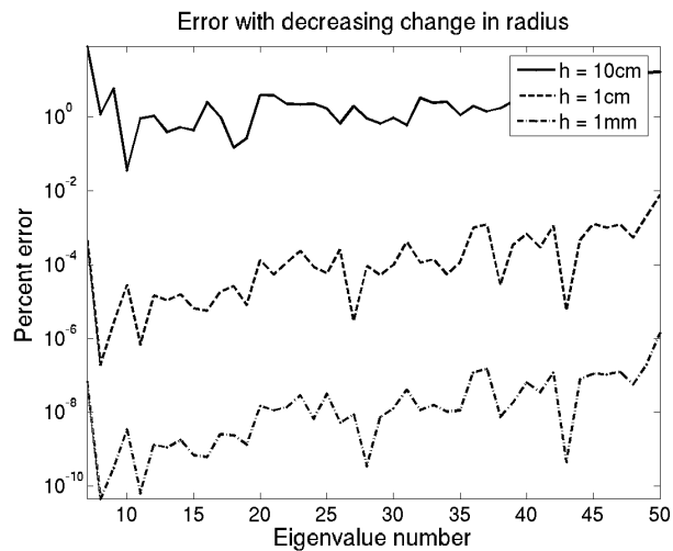
Figure 13: Error for different size h . 4 planes of symmetry.
