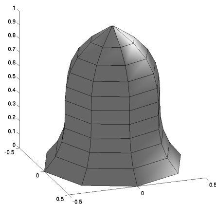
Figure 14: Whole bell geometry, 8 planes of symmetry.
