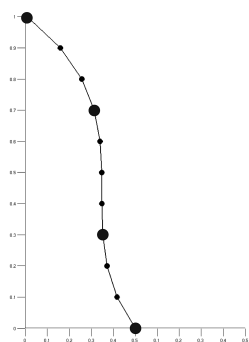
Figure 1: Parametric curve.
